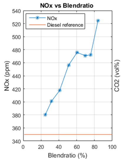
Figure 26: NO x vs. blend ratio with original diesel injection timing.
