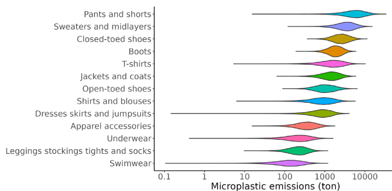
Figure S.16 Baseline emissions of microplastics from clothing and footwear categories to the environment for the EU (2050).
