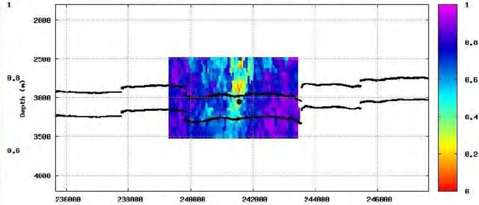
CORRVL, slice at Y-Easting 241550m event:42 binnul:13
