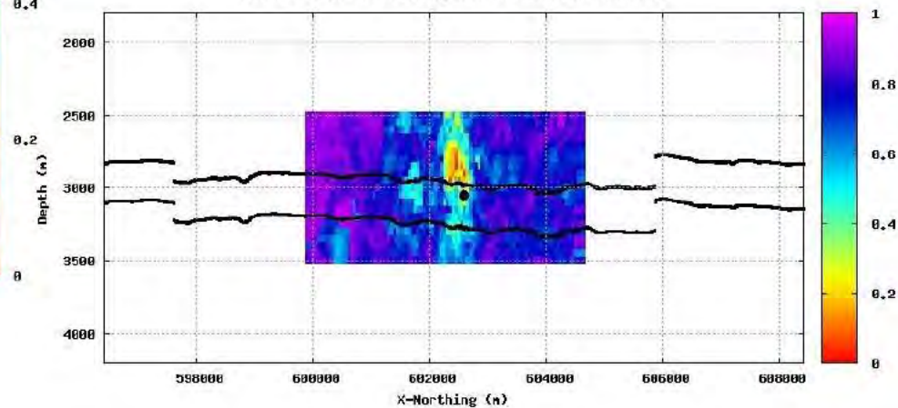
CORRVL, slice at Y-Easting 241550m event:42 binnul:13
