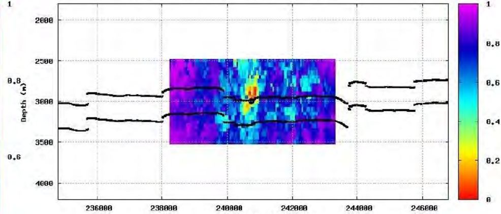
CORRVL, slice at Y-Easting 240750m event:34 binmul:10
