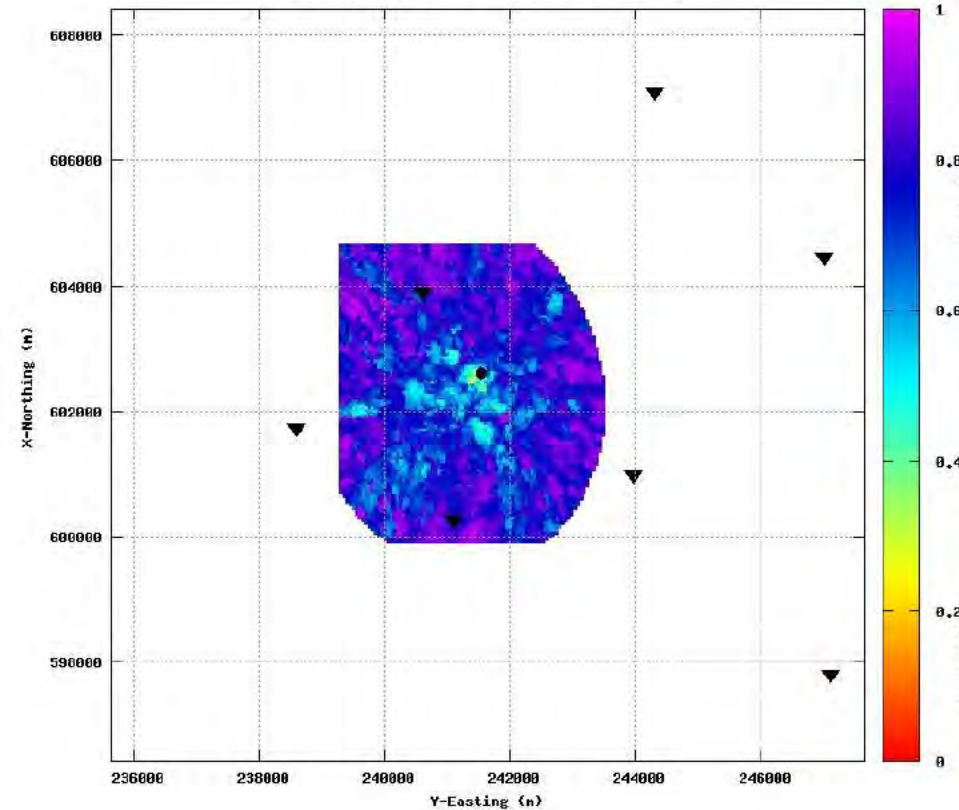
CORRVL, depth slice at ZSHI=3850m event:42 binnul:13
