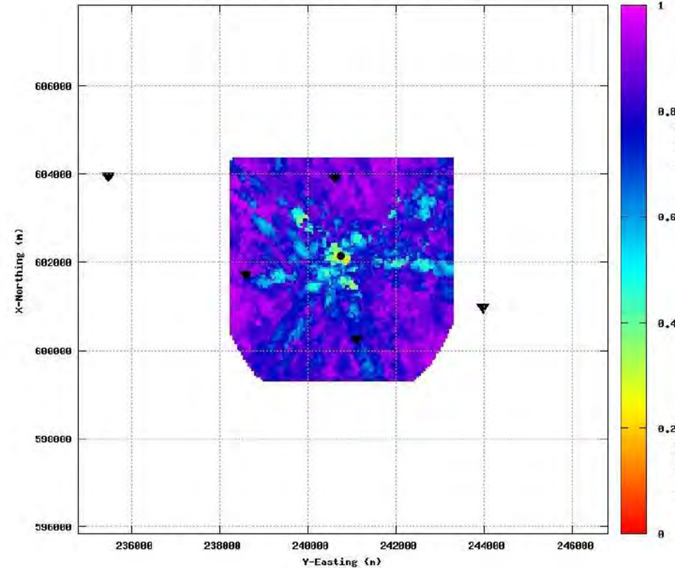
CORRVL, depth slice at ZSHI=3880m event:34 binmul:10
