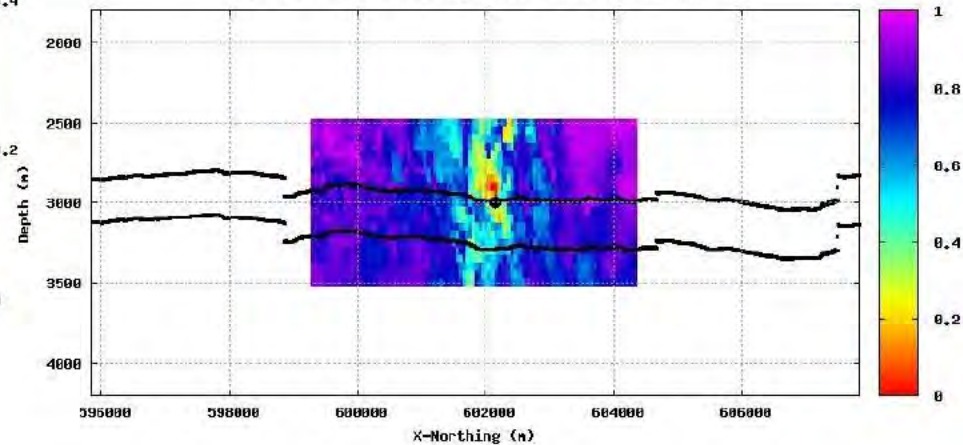
CORRVL, slice at Y-Easting 240750m event:34 binmul:10
