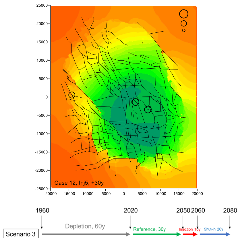
Figure 4.4: Seismic catalogue associated to Scenario 3 (source: Dynafrax).
