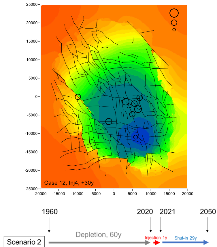
Figure 4.3: Seismic catalogue associated to Scenario 2 (source: Dynafrax).
