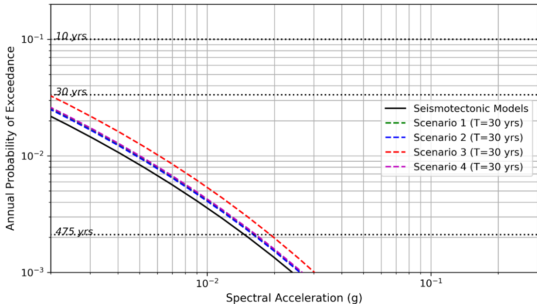
Figure 8.2: Groningen Reservoir site – Top: Mean seismic hazard curves calculated with a period related to the injection time only ( T=1, 5, 10 years). Bottom: Mean seismic hazard curves calculated with a period related to the injection time + shut-in period ( T=30 years) – Horizontal component, V_{S30} = 200 m/s, 5 % damping. Induced GMPE: Bommer et al. 2016. Note: the return periods are shown only for information and they can only be considered for the seismotectonic model.
