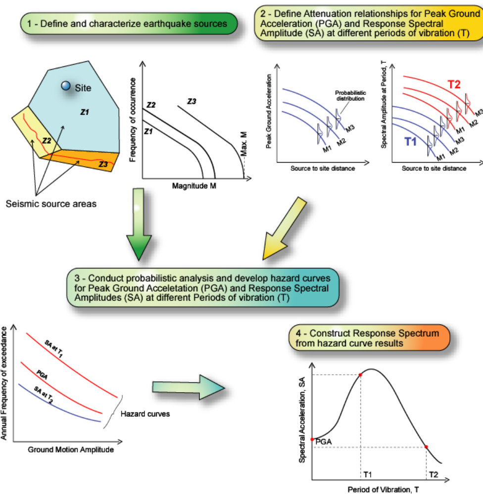
Figure 3.1: Probabilistic seismic hazard method flowchart.
