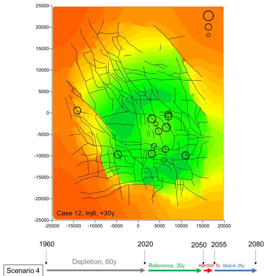
Figure 4.5: Seismic catalogue associated to Scenario 4 (source: Dynafrax).
