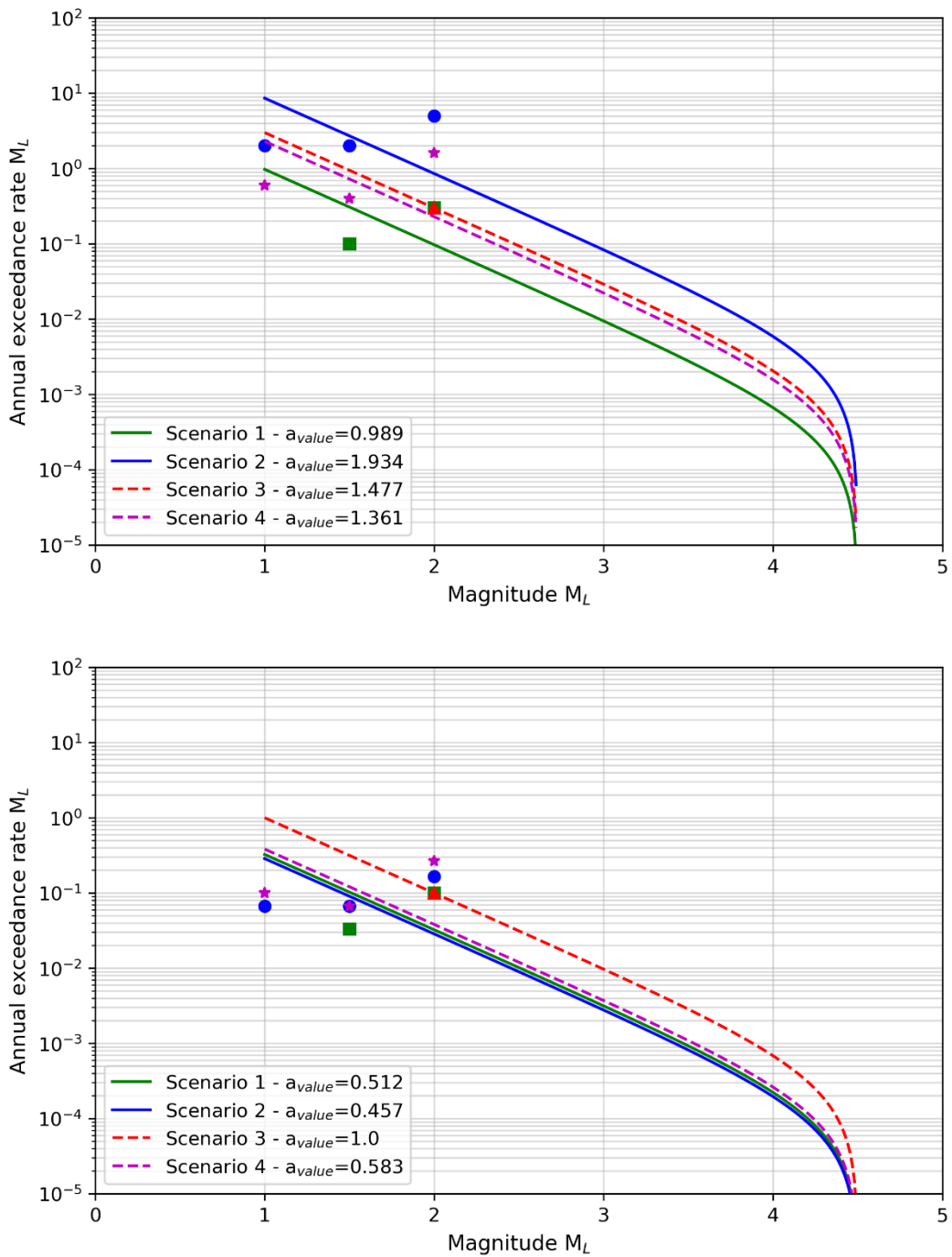
Figure 6.2: Gutenberg-Richter models for the four scenarios (1-2-3-4) with a mean a -value of all the different Mfit (1.0, 1.5 or 2.0 depending on the scenarios). Top: rates calculated over the injection time only (1, 5 or 10 years depending on the scenarios). Bottom: rates calculated over the injection time + shut-in period (30 years for all scenarios).
