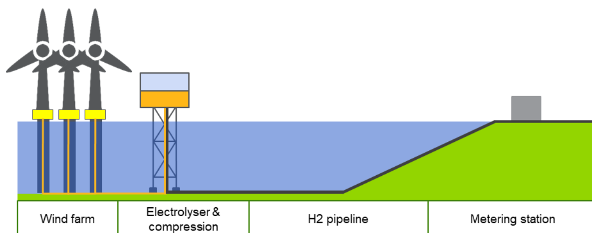
Figure 4-4 Configuration 4 – off-grid centralised electrolysis
