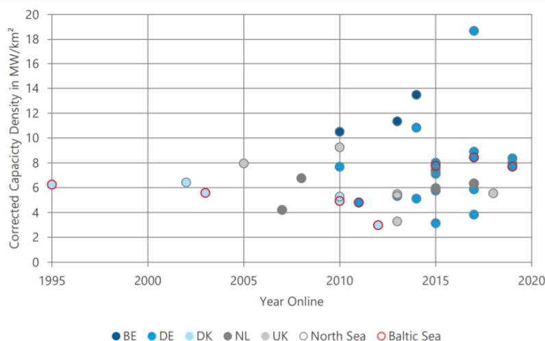
Figure 7-1: Overview of capacity densities of wind farms (Deutsche WindGuard) 141
