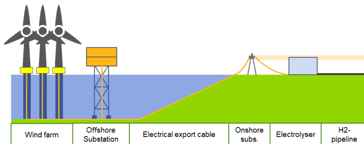
Figure 4-1 Configuration 1 – on-grid electrolysis
