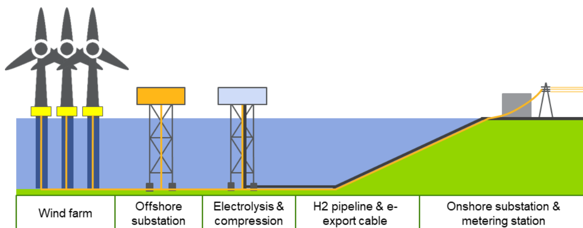
Figure 4-5 Configuration 5 – hybrid centralised electrolysis
