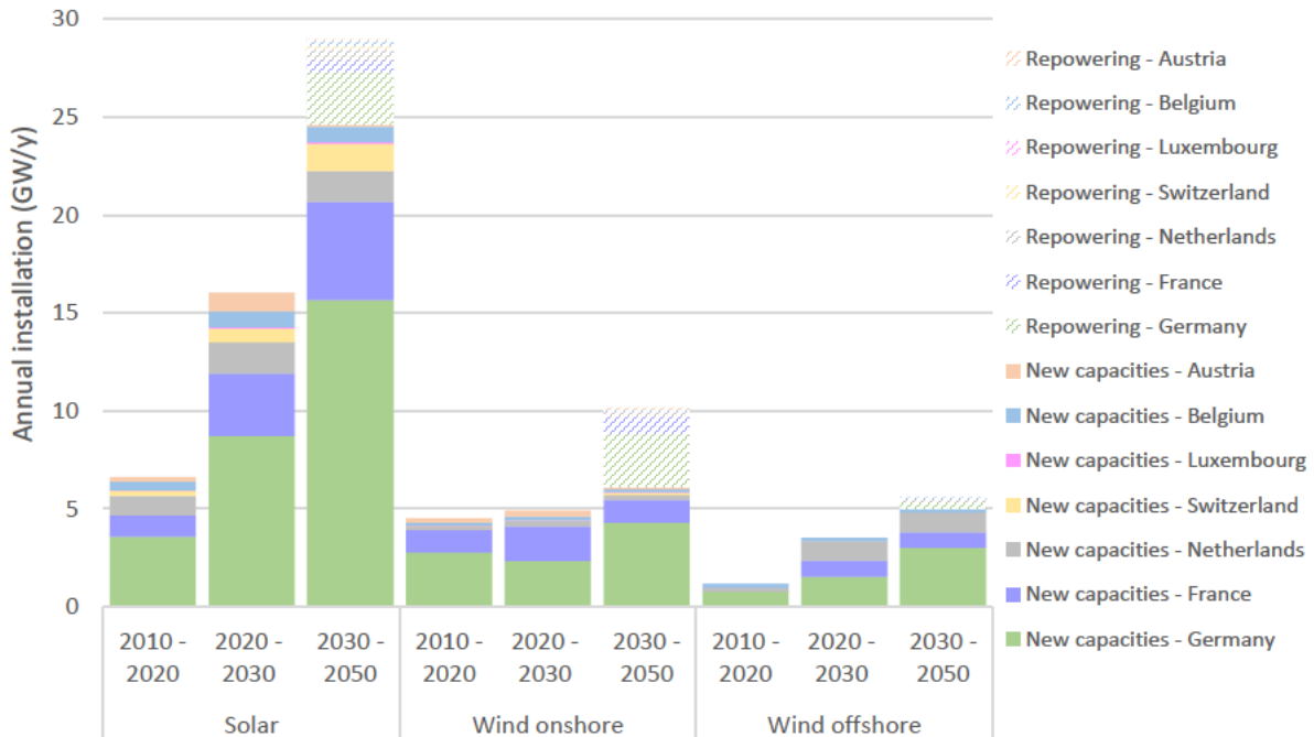
Figure 21 - Evolution of annual vRES installation rates (GW/y) 20 . Source: own illustration.
