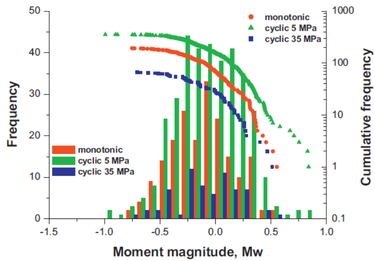
Figure 3-6: Magnitude frequency distribution of the seismic event moment magnitude resulting from hydraulic fracturing – hydraulic stimulation modelling of geothermal reservoir rock mass (Fig.10 in Yoon et al. 2014).
