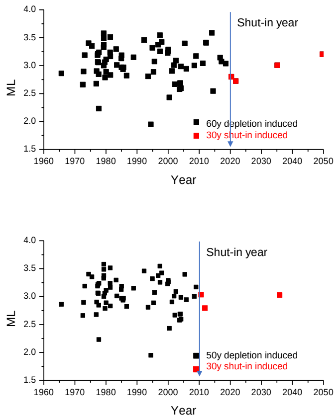
Figure 6-3: ML of simulated seismic events plotted against time, (top) shut-in scenario 1, (bottom) shut-in scenario 2. The vertical line denotes the shut-in year.
