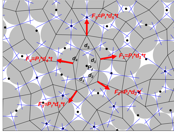
Figure 3-2: Pore network model. Flow channels (blue lines at the particle contacts) connect two neighboring pore spaces bounded by polygons. Black dots at the polygon centers are virtual pores where pressure ( P_f ) is stored. Red arrows are resultant forces applied to the particles surrounding the pore space due to the pore fluid pressure P_f (Fig.2 in Yoon et al. 2014).
