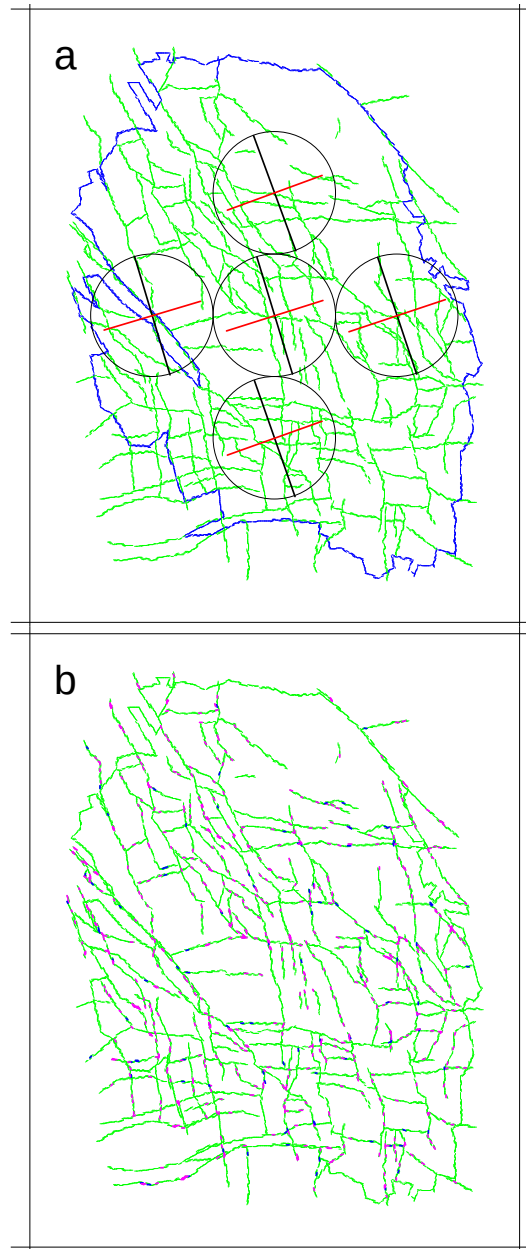
Figure 4-4: (a) PFC2D Groningen gas field model, where the in-situ stress field was initialized: SH_{max} = 50 MPa, Sh_{min} = 40 MPa and the orientation of SH_{max} is N160E. (b) distribution of smooth joint failures ( blue : Mode I tensile failure, magenta : Mode II shear failure) resulting from initialization with an anisotropic in-situ stress field.
