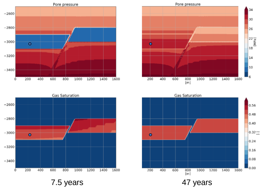
Figure 7-6: State after 7.5 years and 47 years injection of CO2. Dots are injection points.
