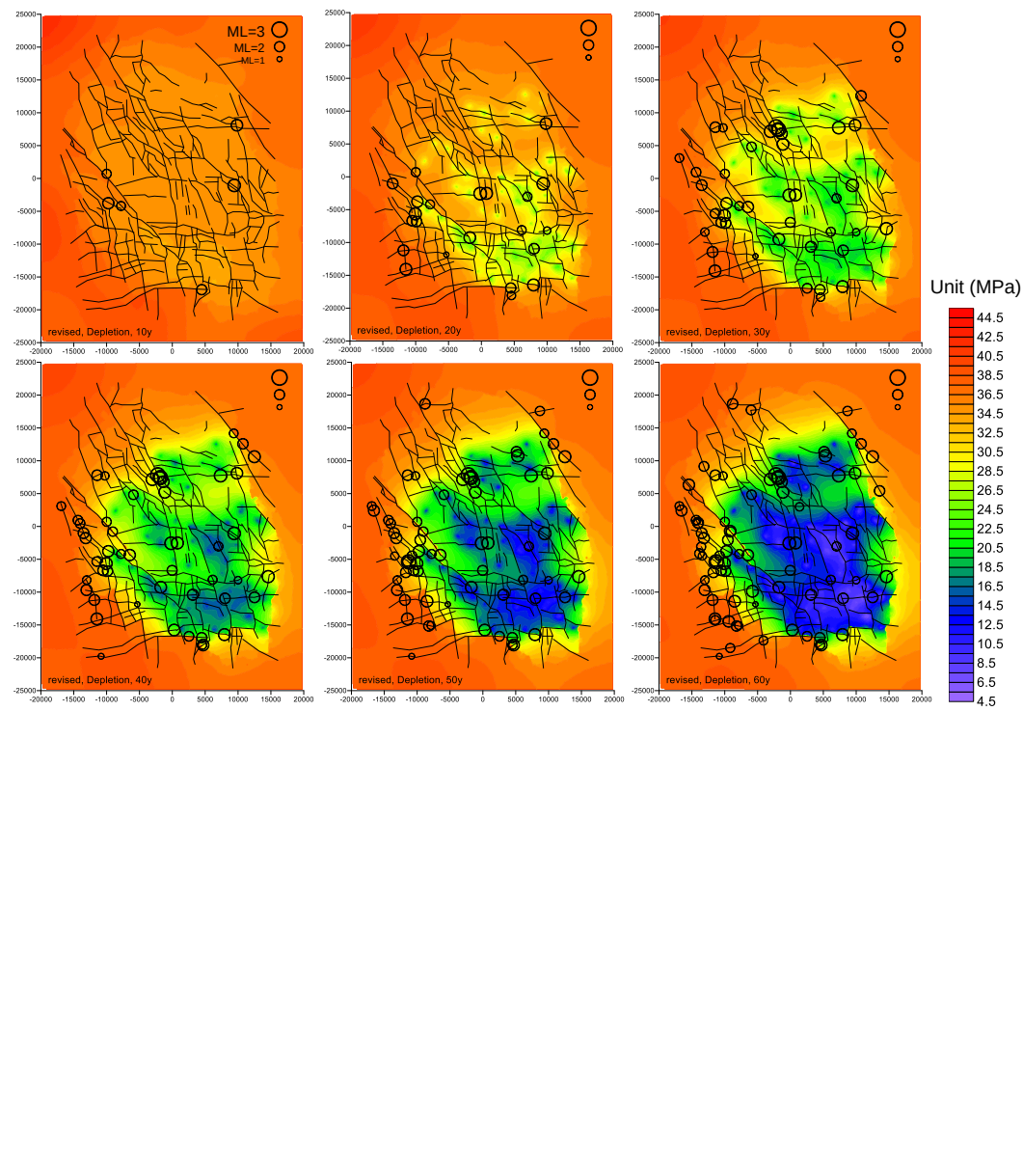
Figure A-1: Evolution of reservoir pressure and seismicity simulated by the depletion model (date 2021 November 24). Results for every 10 years after the start of simulated depletion are shown. The axes show the distance (in meters) from the center of the study region.
