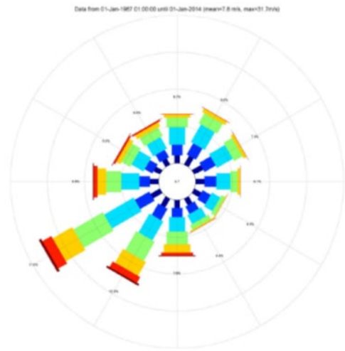
Figure A2.1 - Annual wind rose plots from metocean reports of Borssele II, HKZ, HKN and HKW.
