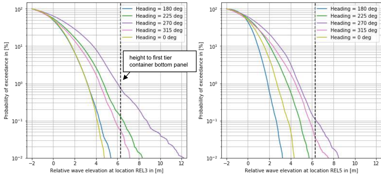
Figure 3-30: Cumulative distribution of the relative wave elevation, H_s = 4.5 m / T_p = 8.5 s, beam waves Configuration 2, left: location REL 3 (amidships), right: location REL 5 (bow). The vertical dash line denotes the height to freeboard deck and container bottom panel
