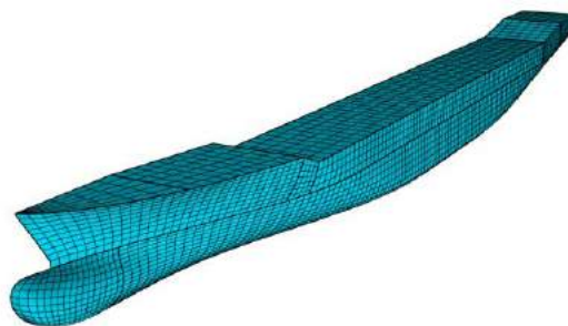
Figure 3-40: Hull form of the feeder used for the computations
