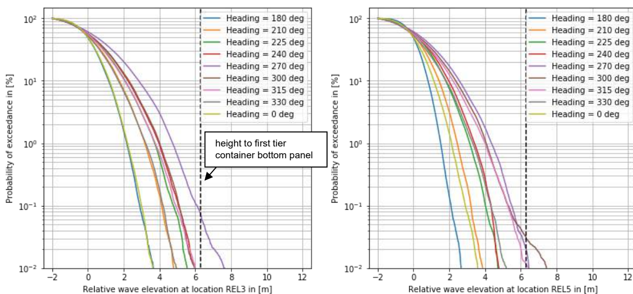
Figure 3-29: Cumulative distribution of the relative wave elevation, H_s = 3.0 m / T_p = 7.0 s, beam waves Configuration 2, left: location REL 3 (amidships), right: location REL 5 (bow)
