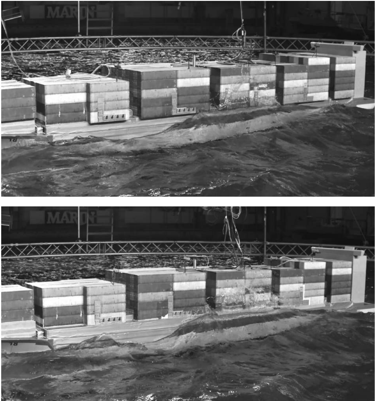
Figure 3-26: Wave impact observed in wave condition H_s = 4.5 m, T_p = 8.5 s, \mu = 270 deg (beam waves), time stamp 479 s from start official measurement Top: configuration 3, bottom: configuration 6
