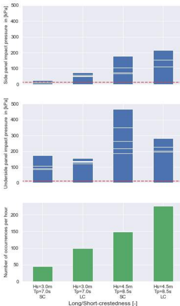
Figure 3-21: Stacked-up representation of the top five transverse wave load pressures (top), top five vertical wave load pressures (middle) and hourly number of occurrences (bottom) Variation in crest character Beam waves, depth 21.3 m
