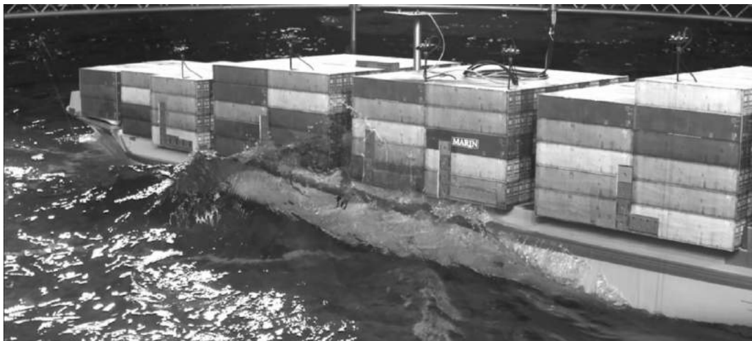
Figure 3-17: Green water load from in stern-quartering waves
