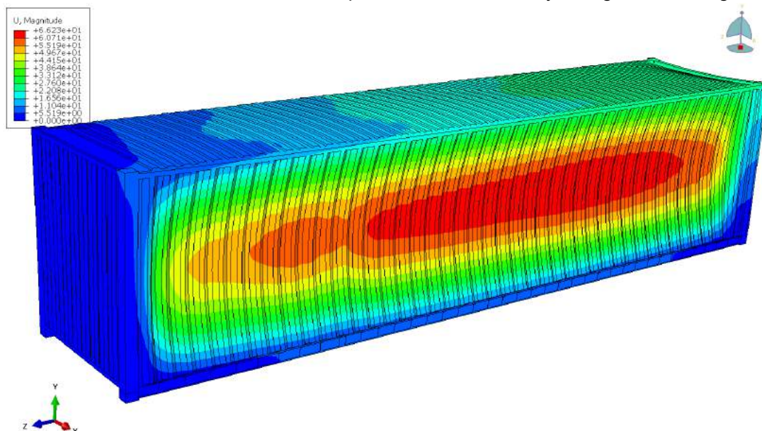
Figure 3-9: Max. full scale displacement in [mm] as determined by FE simulations in the previous study
