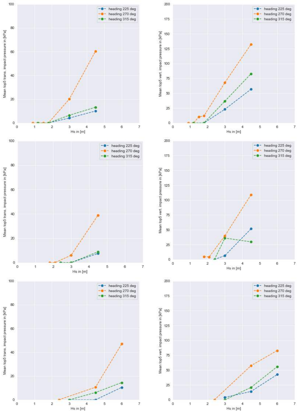
Mean top 5 wave pressure loads; From top to bottom: configurations 1, 2 and 3
