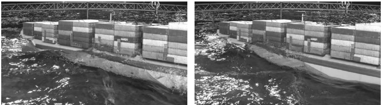
Figure 3-31: Takes of the largest transverse and vertical impact from green water taken shortly after each other, configuration 2, H_s = 4.5 m, T_p = 8.5 s, heading 315 deg
