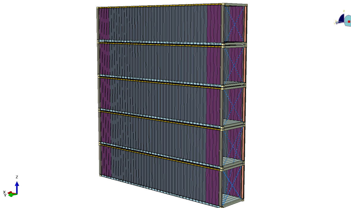
Figure 5-1: Geometry model of the container stack with 5 containers
