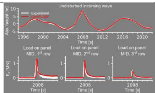
Extreme event matching applied to determine local and global wave impact loading on the breakwater of a container vessel (courtesy of the CRS working group green water).
