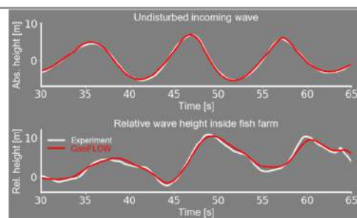
Extreme event matching applied to obtain local pressure distributions during internal sloshing inside a floating fish farm (courtesy of Viewpoint Seafarm AS - Spider Cage concept).
