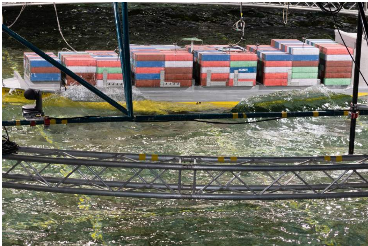
Photo 14 Test 33327_01OB_04_004_009_01: \mu = 270^\circ – H_s = 4.5 m – T_p = 8.5 s
