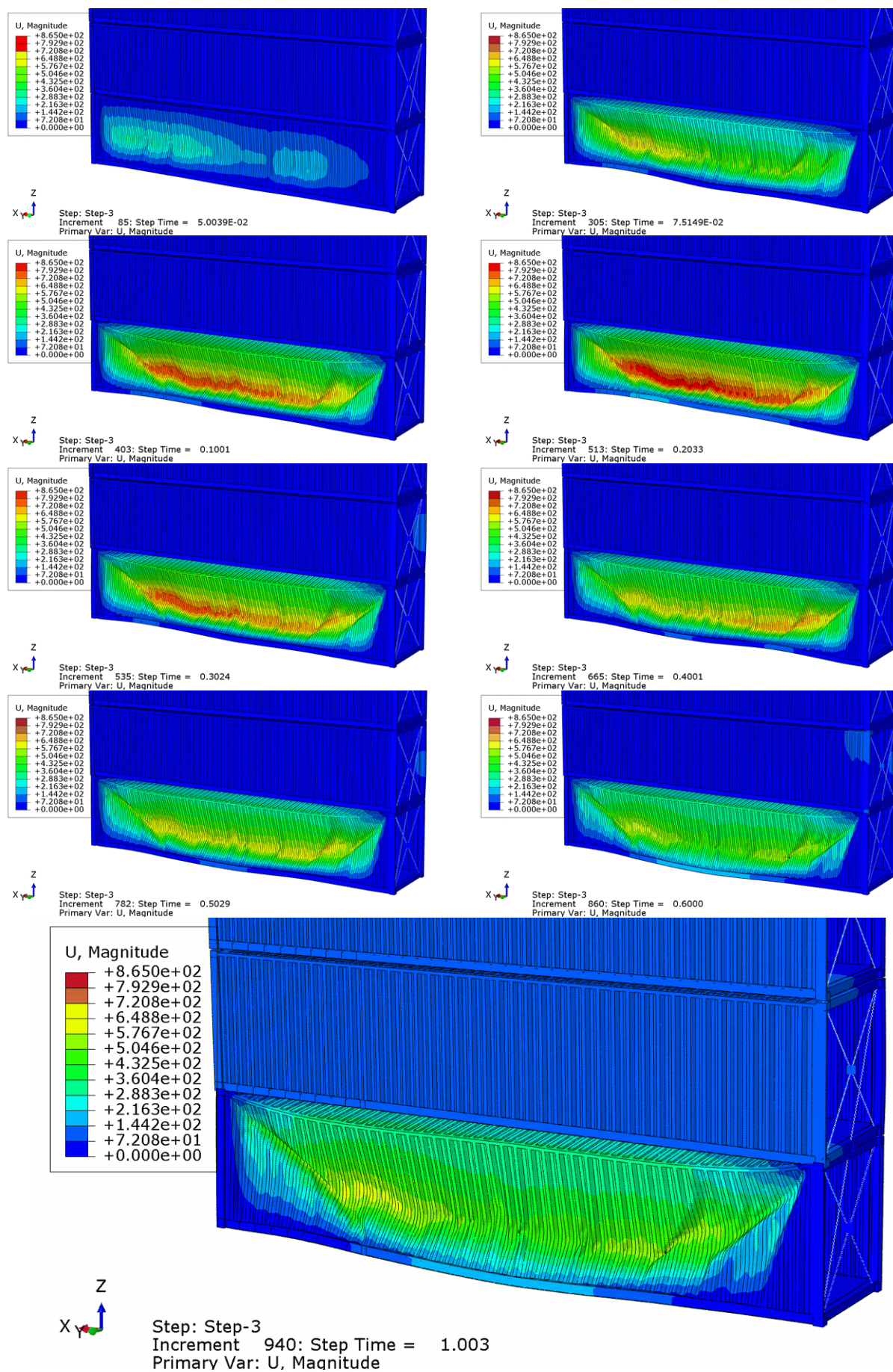
Figure 5-12: Simulation 2-4 (Beam seas), Deformation of the container at different time steps (top) and residual damage and displacement values at the end (bottom)
