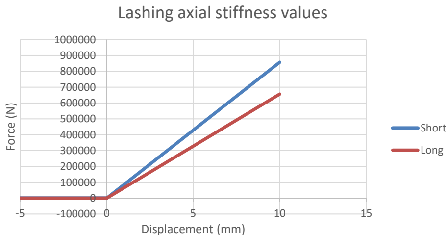
Figure 5-7: Lashing stiffness values
