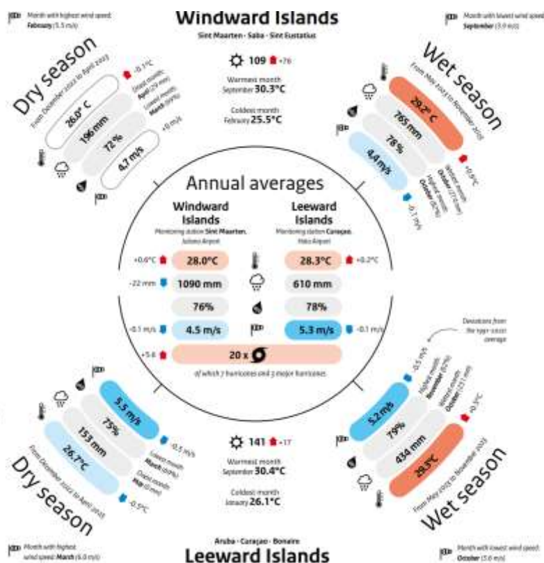
Figure 2. Deviation of weather parameters of the year 2023 from the long-term average (1991-2020). In 2023, the dry season (December-April) was wetter and colder than the long-term average, while the wet season was dryer and warmer for all Dutch islands in the Caribbean (KNMI, 2023).
