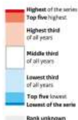
Figure 2. Deviation of weather parameters of the year 2023 from the long-term average (1991-2020). In 2023, the dry season (December-April) was wetter and colder than the long-term average, while the wet season was dryer and warmer for all Dutch islands in the Caribbean (KNMI, 2023).
